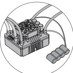
External Capacitor Module (also called CapPack) Wiring
